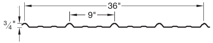
PBU Panel
