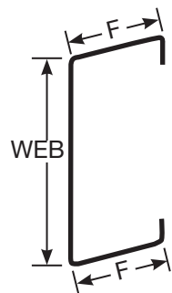
Eave Strut double broke, low side
