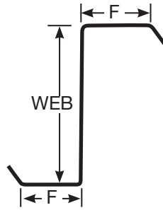
Zee Purlin
